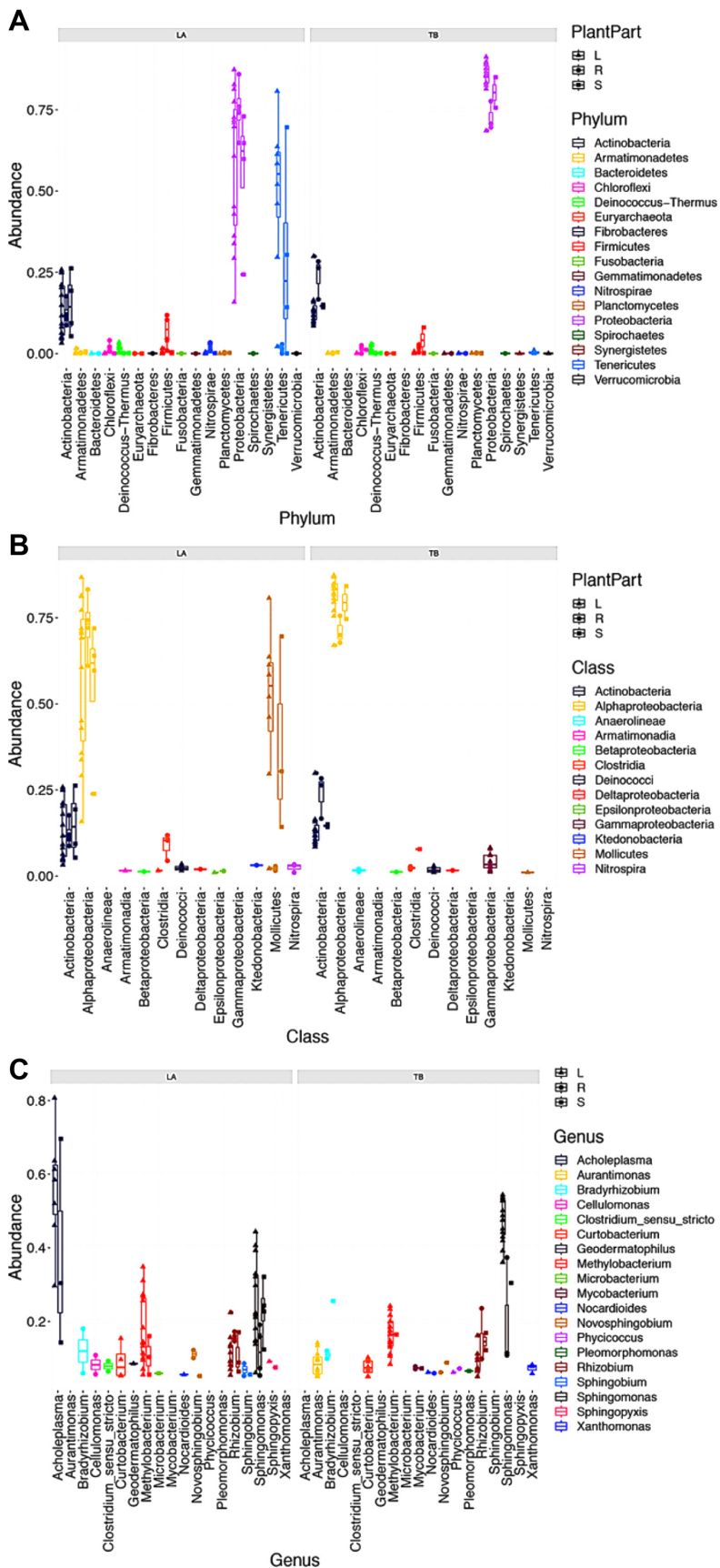
Supplementary Fig. 2. Taxonomic composition and relative abundance of dominant bacterial phyla (A), classes (relative abundance > 0.01) (B), genera (relative abundance > 0.05) (C) in the different plant compartments (L, leaf; R, root; S, stem) of the LA and TB cultivars.
