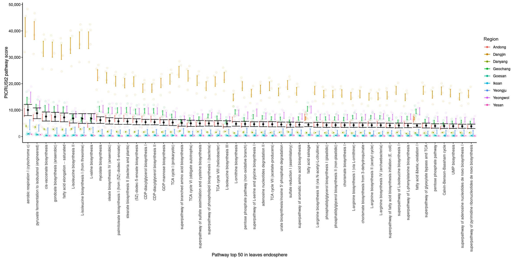
Supplementary Fig. 5. The top 50 predicted pathways in the endosphere of leaves. The black points represent the average, and the error bars represent the standard deviation for all regions. PICRUST2, Phylogenetic Investigation of Communities by Reconstruction of Unobserved States 2.
