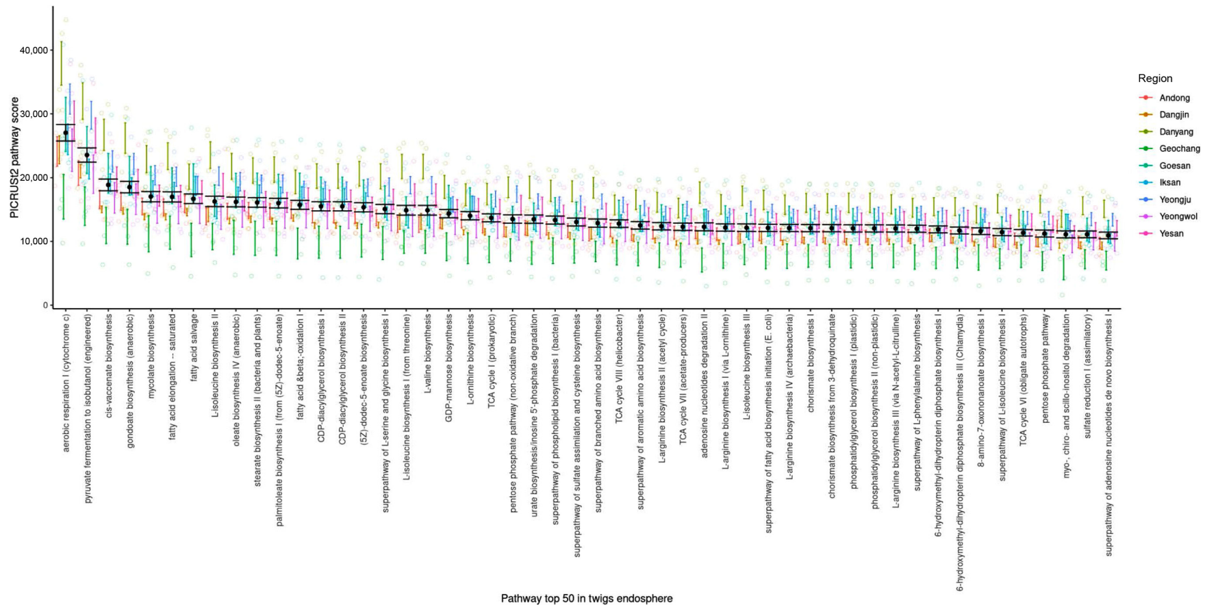
Supplementary Fig. 6. The top 50 predicted pathways in the twig endosphere, with the black dots and error bars representing the average and standard deviation of all region portraits. PICRUS2, Phylogenetic Investigation of Communities by Reconstruction of Unobserved States 2.
