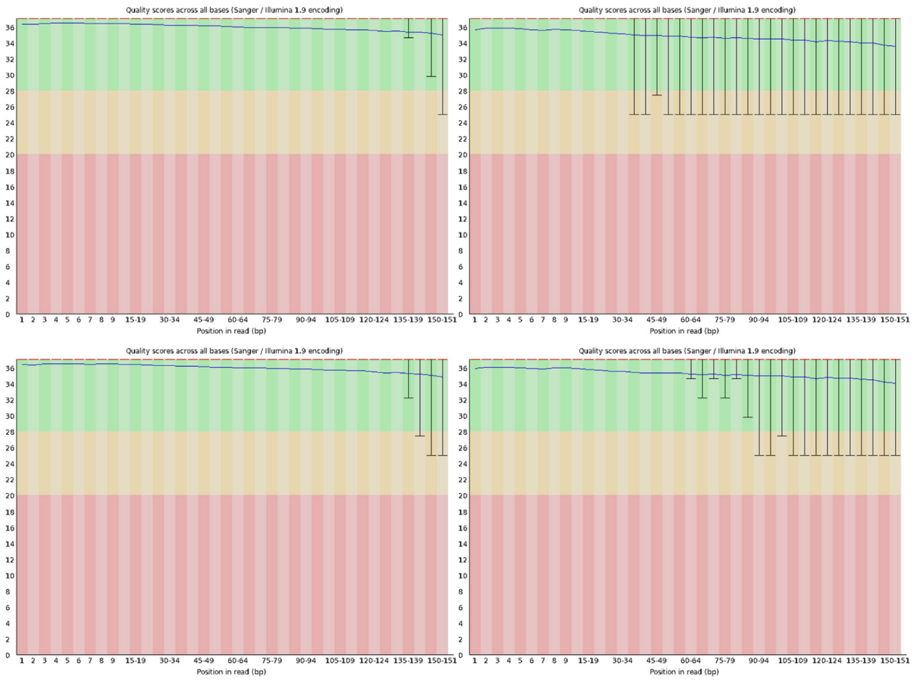
Supplementary Fig. 1. Example of sequencing quality of RNA-seq samples. Per base sequence, the quality of forward and reverse paired-end reads was measured using FASTQC.
