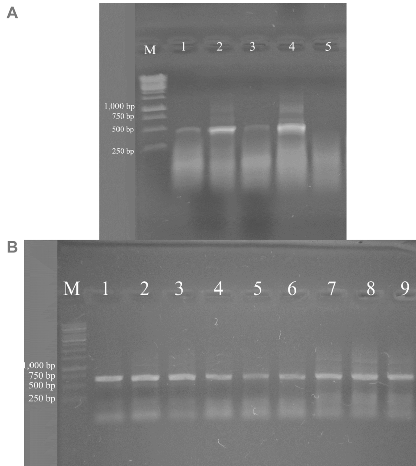
Supplementary Fig. 1. Analysis of PCR products by agarose gel electrophoresis. M, GeneRuler 1 kb DNA ladder (Termofisher). The target-specific band size is around 473 bp for Prunus virus T (A) and 688 bp for cherry virus A (B).
